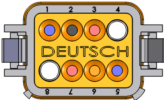
0857-3 Over Current
