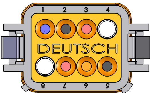
0857-7 Delay on Break
